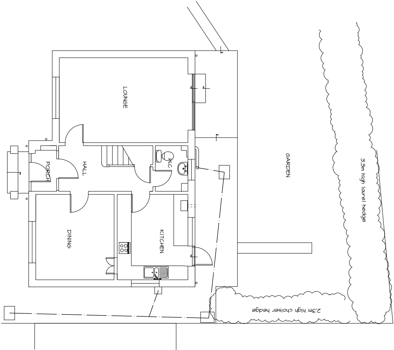
Existing Ground
