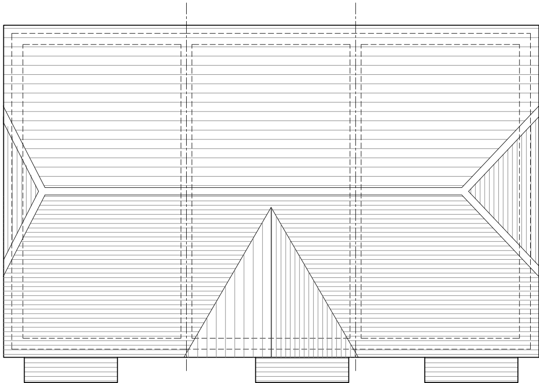
Roof Plan
