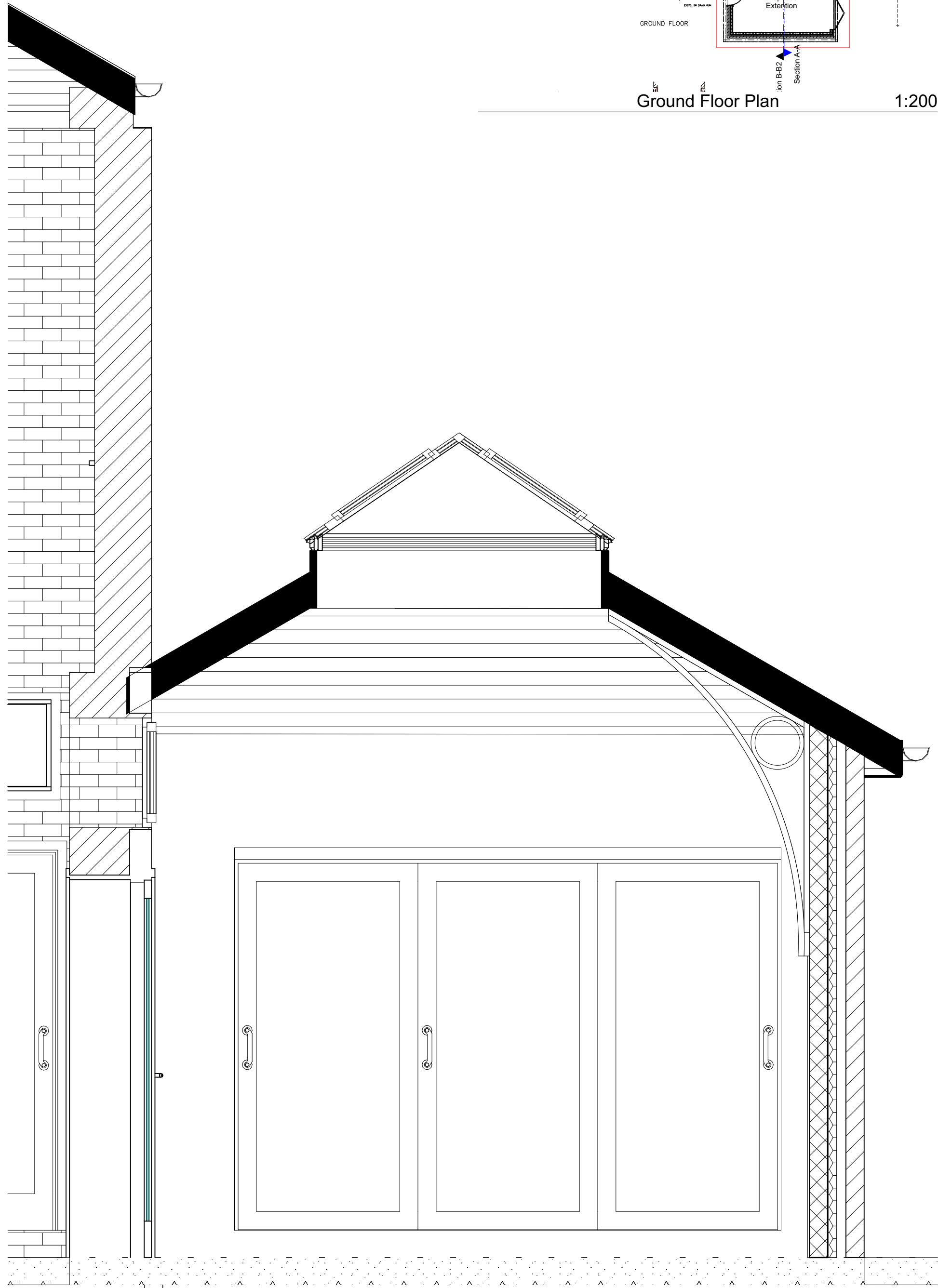
Section A-A Planning 1:20
