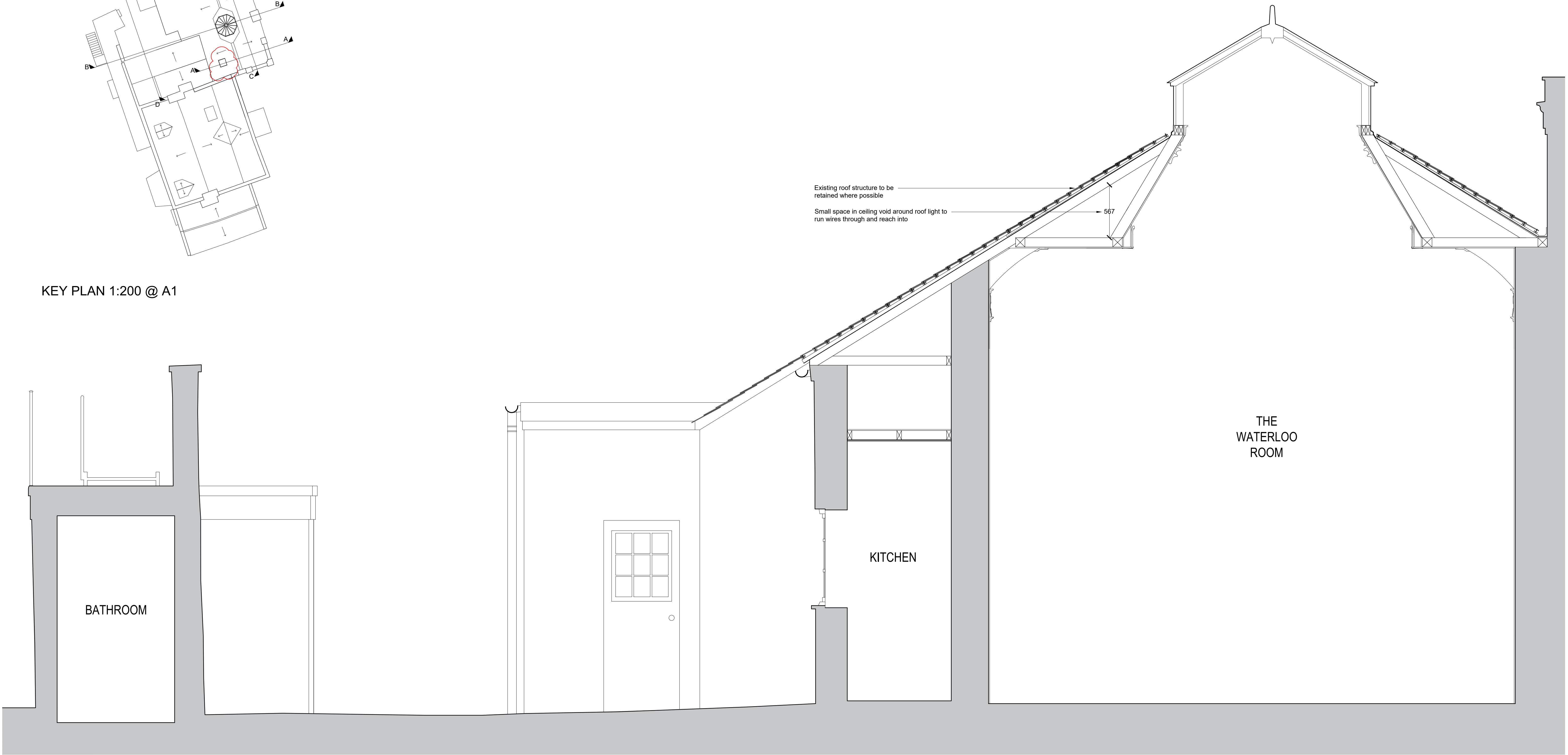
SECTION B-B 1:20 @ A1
