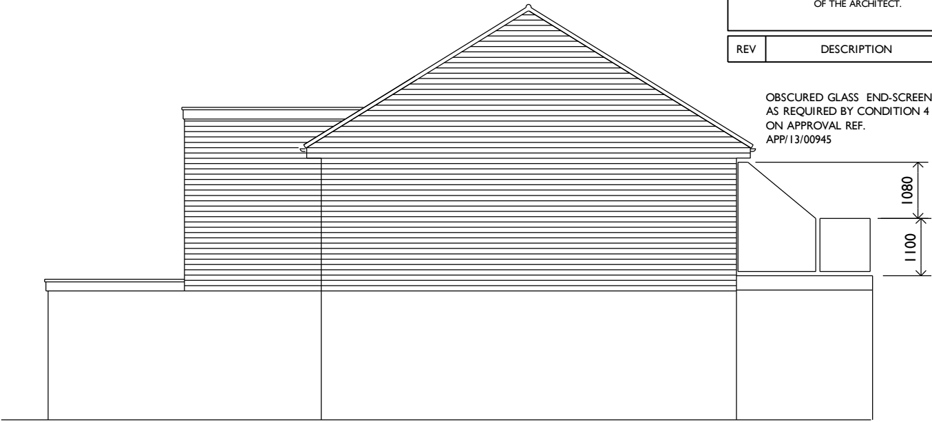
END ELEVATION - WEST
