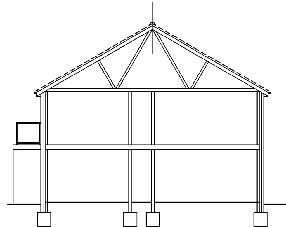
DRAFT SECTION
