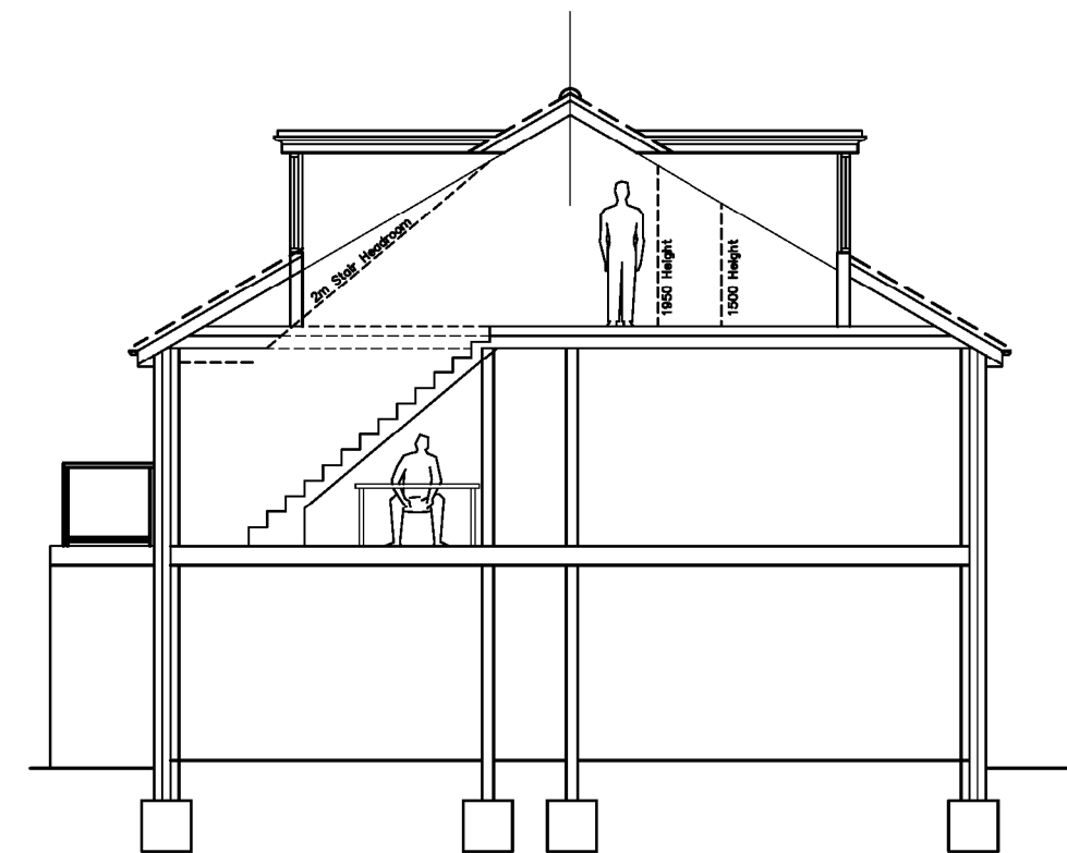
DRAFT SECTION A-A
