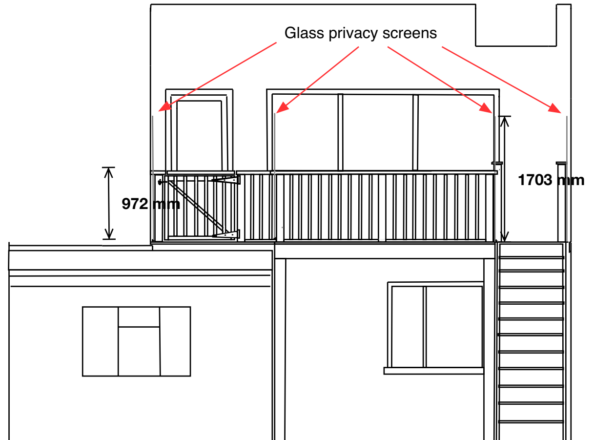
Rear Elevation 1:50
