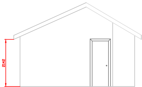
PROPOSED WEST ELEVATION
