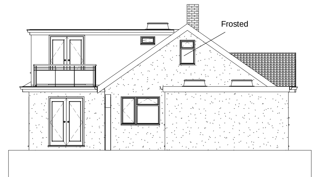
4 West Elevation 1 : 100
