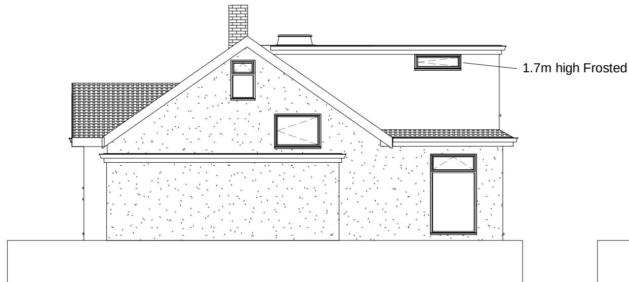
1 East Elevation 1 : 100
