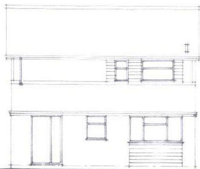
EXISTING ELEVATIONS WEST, Scale 1 : 100 at A3 ( FRONT FACING POOK LANE )
