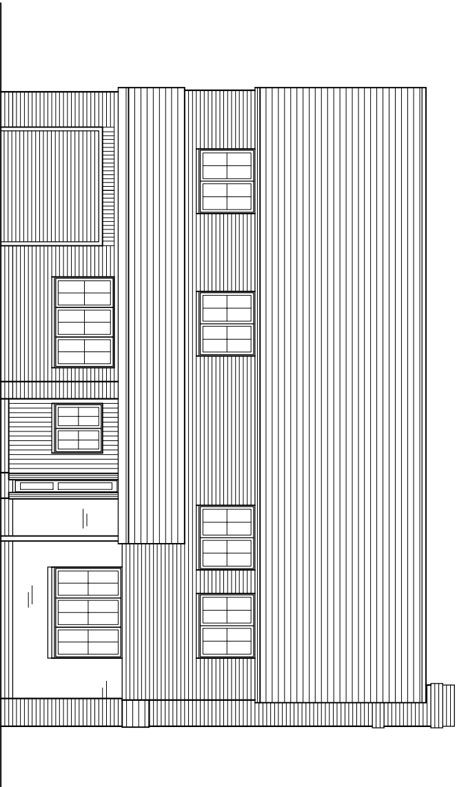
Front Elevation
