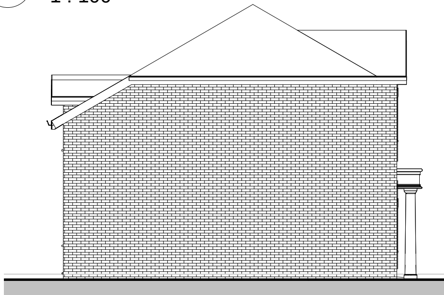
5 Elevation North HT C 1 : 100
