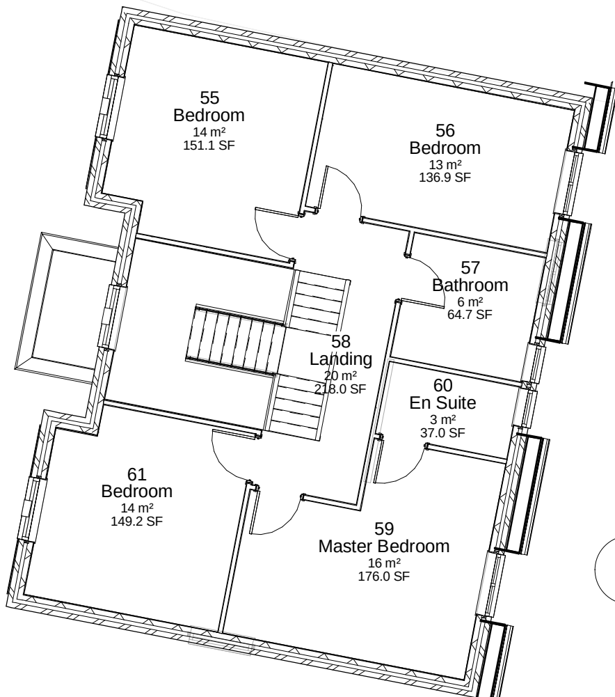
2 First Floor House Type C 1 : 100
