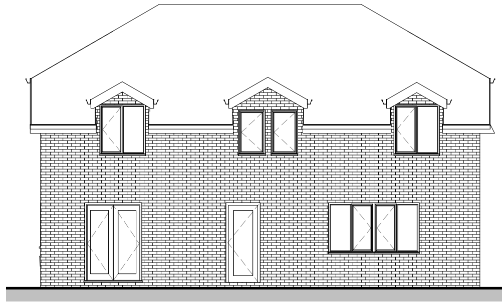
4 Elevation East HT C 1 : 100
