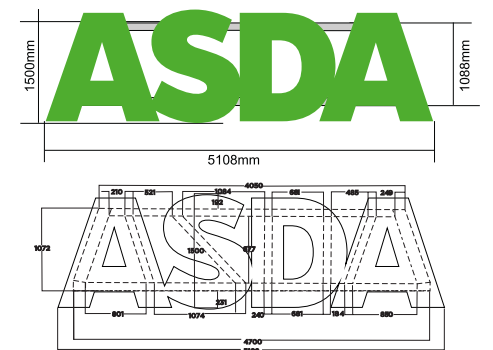
STEELWORK FOR 1500MM ASDA LETTERS WITHOUT FEET
