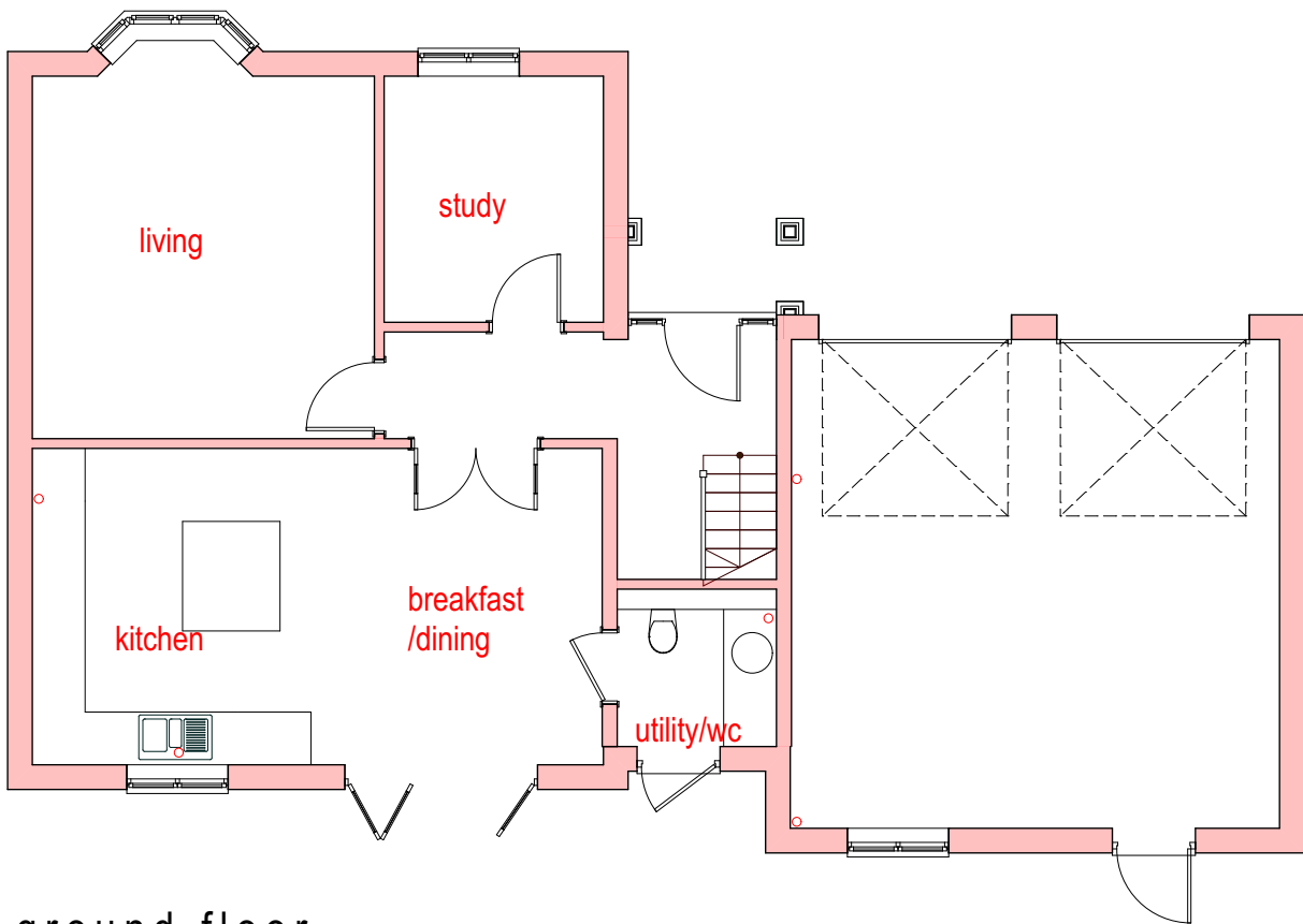
ground floor plot 3 1915ft 2
