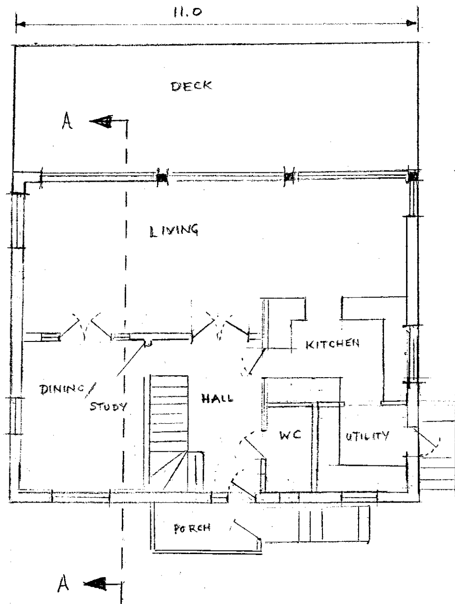
GROUND FLOOR
