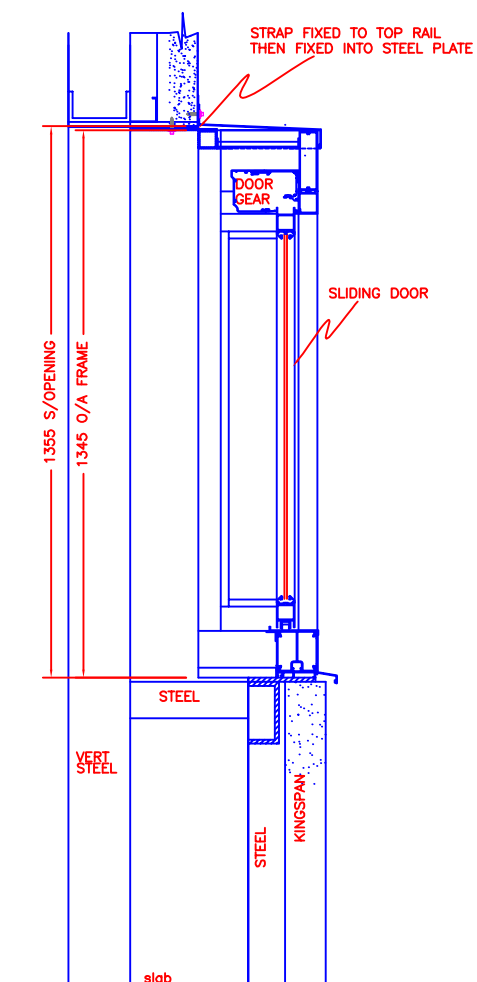
SECTION THRU AT SLIDING DOOR
