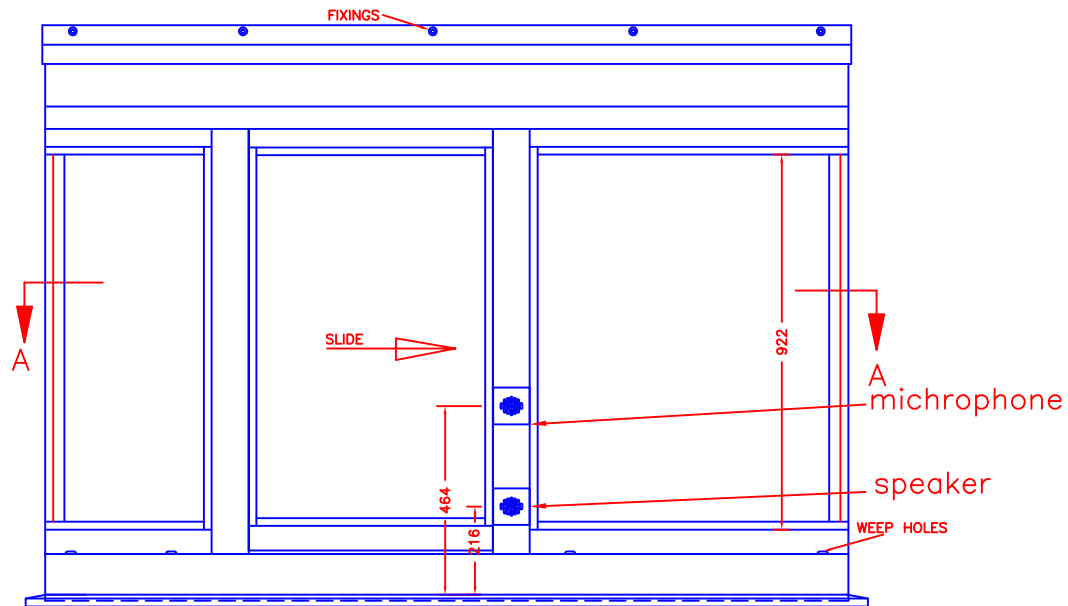
FRONT ELEVATION WITH HOOD APPLIED
