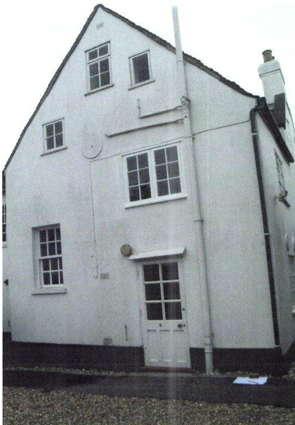
Rear elevation showing the area of the proposed extension and modern door and frame to be removed.
