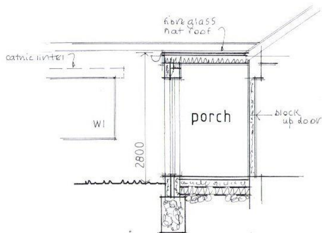
section b-b
