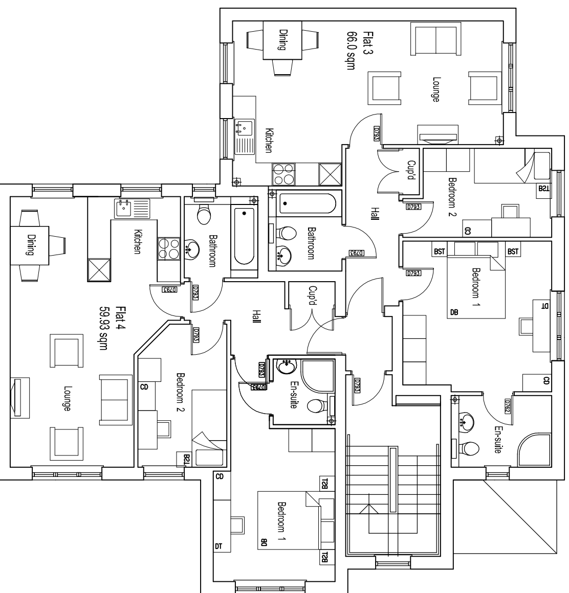
FIRST FLOOR
