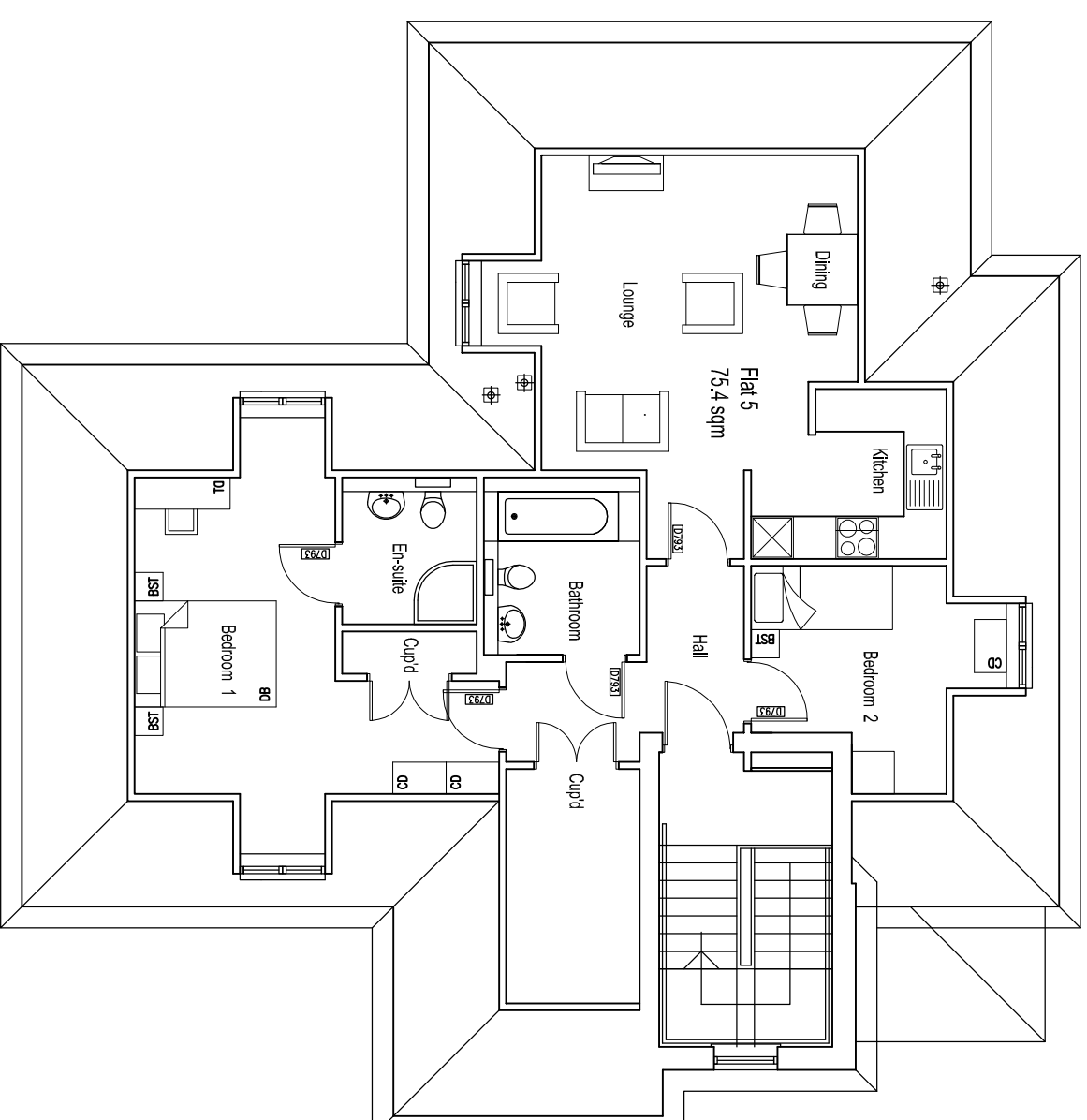
SECOND FLOOR
