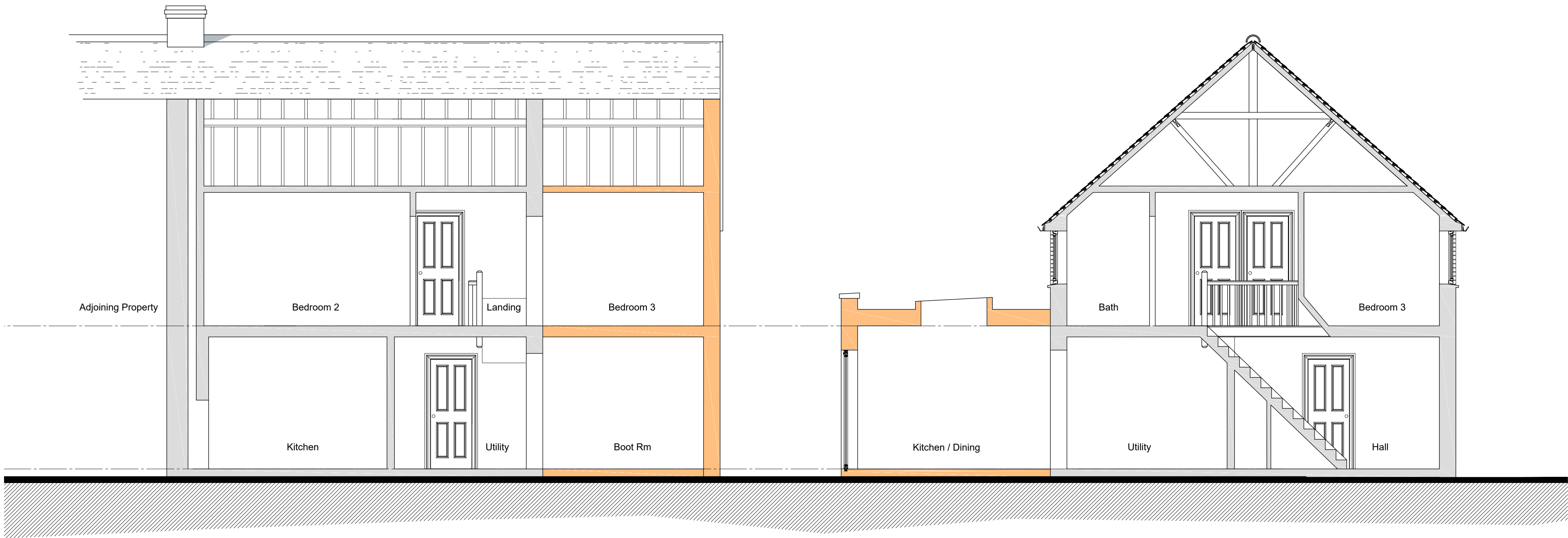
PROPOSED LONG SECTION
