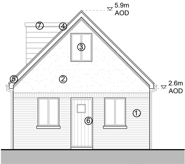
WEST ELEVATION
