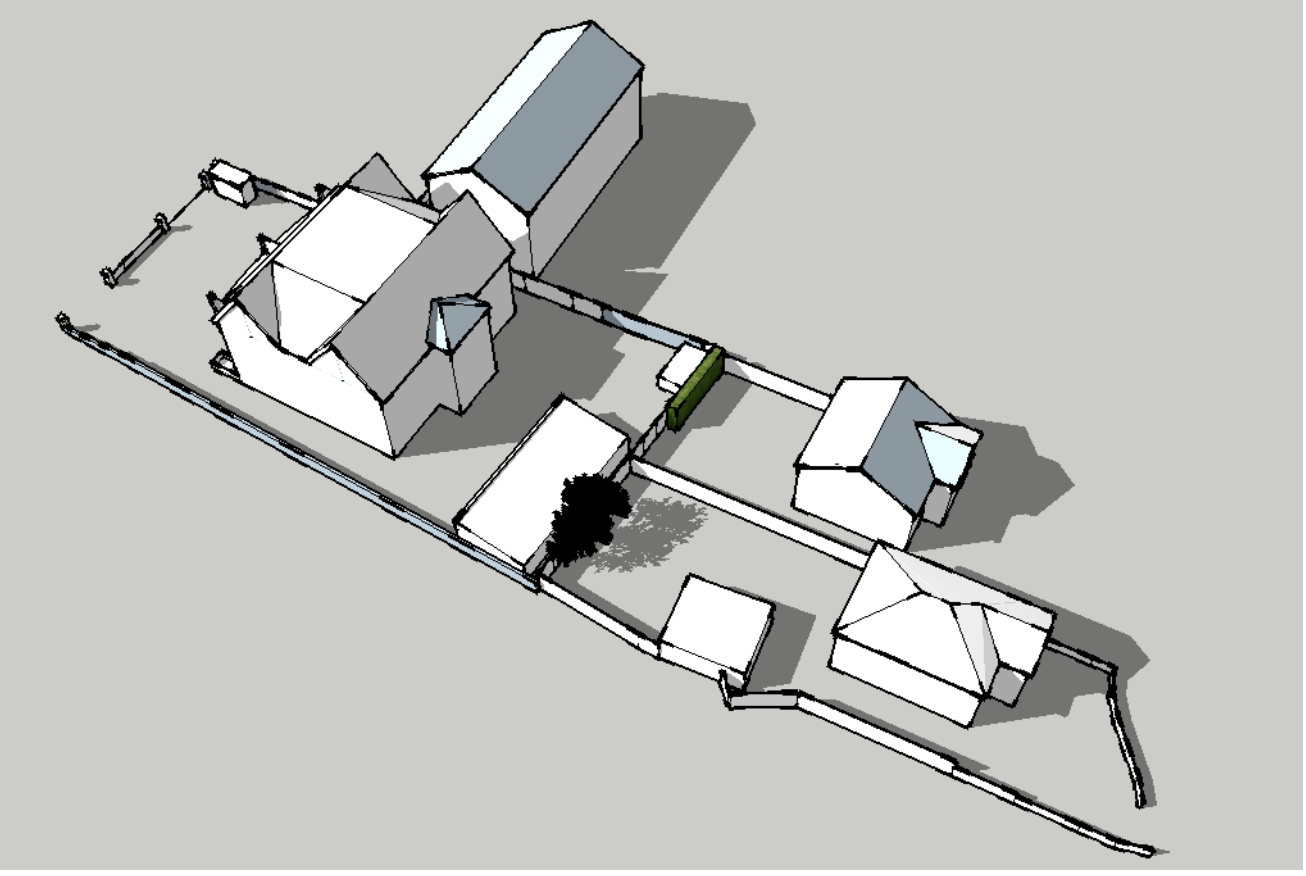
Perspective Of Proposed Building & Neighbouring Buildings Shadows Cast At 11 O'Clock AM On 21st March
