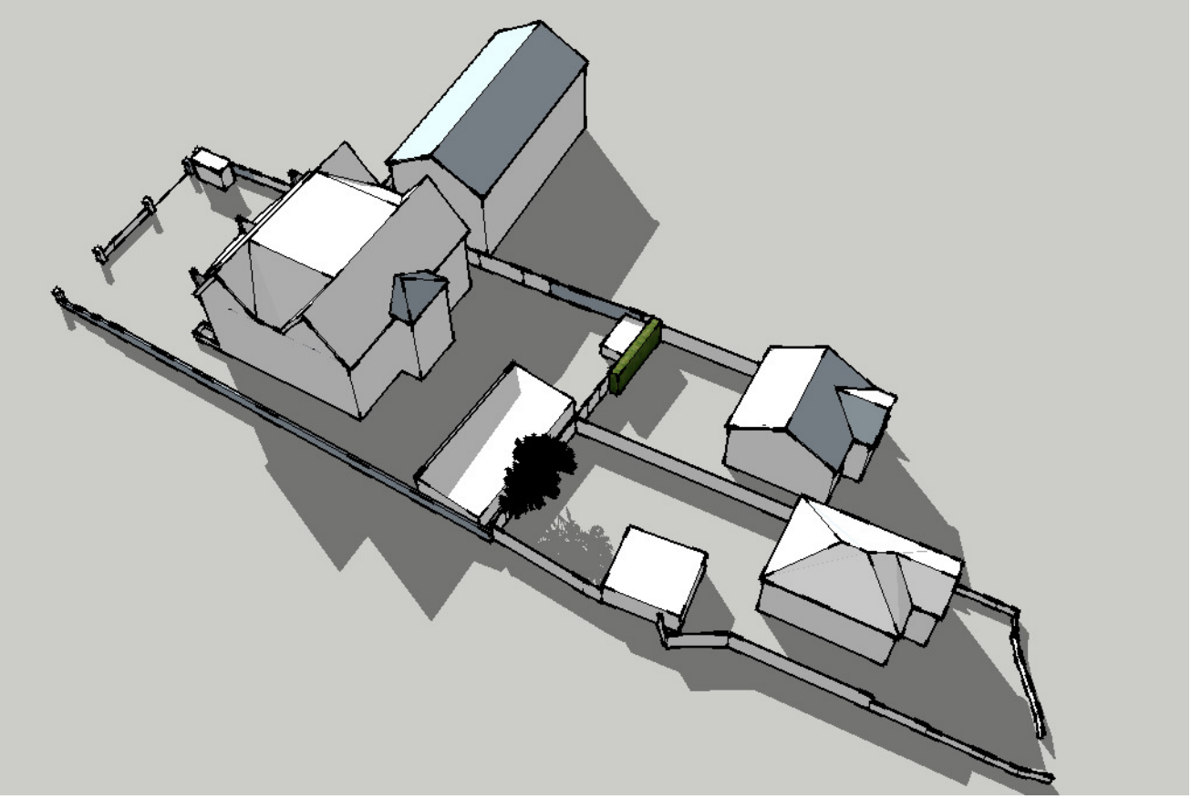
Perspective Of Proposed Building & Neighbouring Buildings Shadows Cast At 3 O'Clock PM On 21st March
