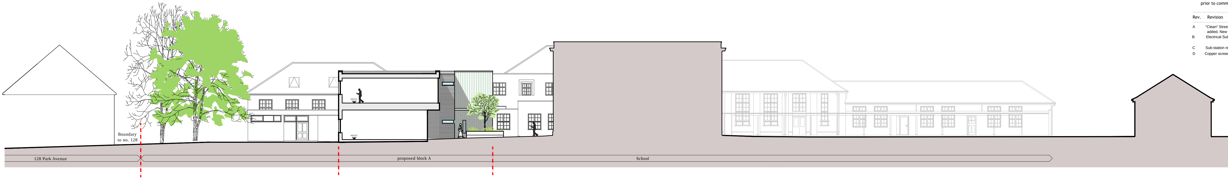
Proposed Site Section through Block A 1:200
