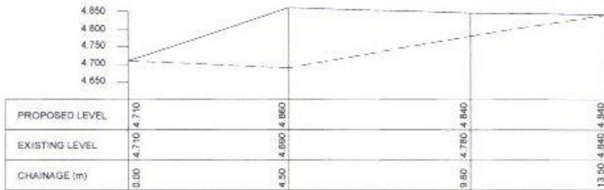
SECTION A-A HORIZONTAL 1:50, VERTICAL 1:5
