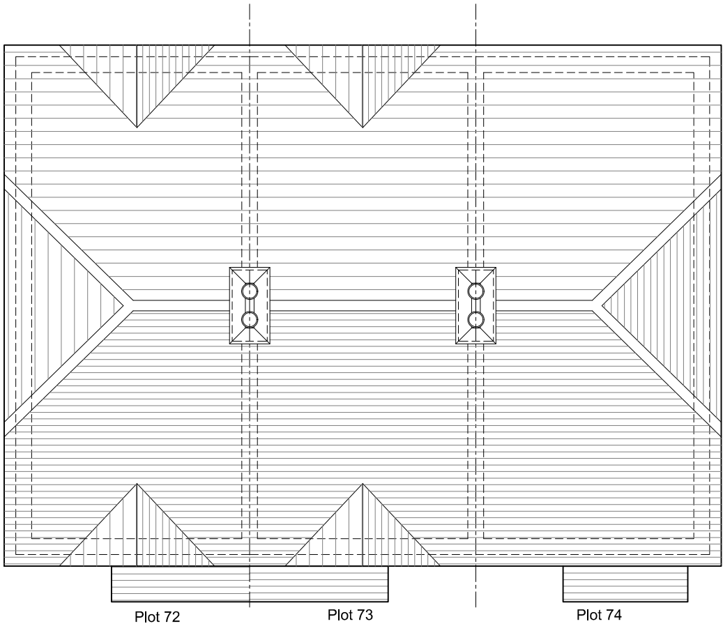
Roof Plan
