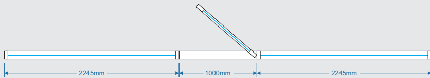
Proposed Shopfront Plan View
