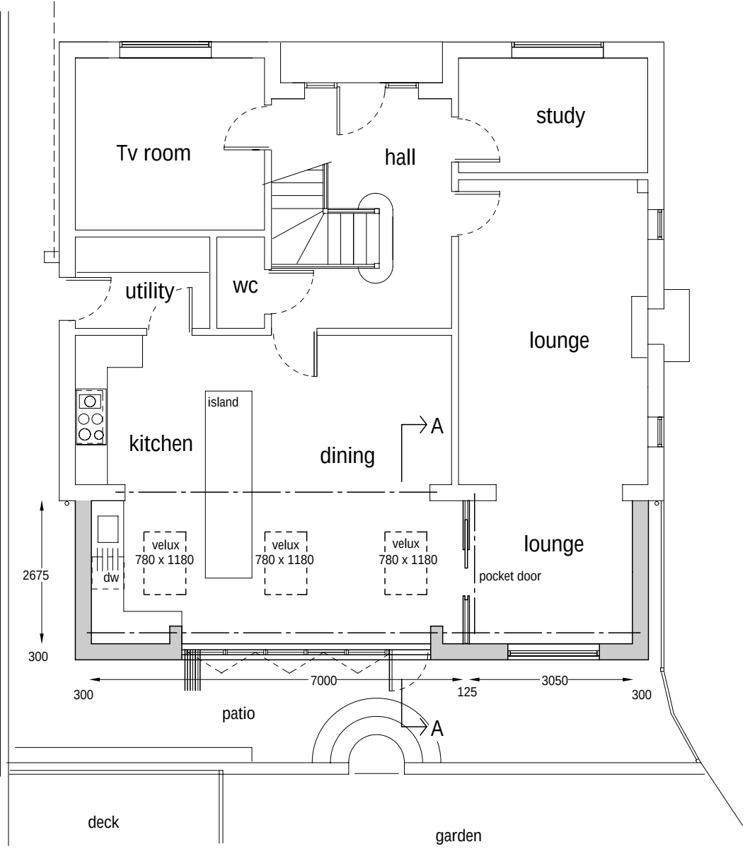
Prop. Ground Floor Plan
