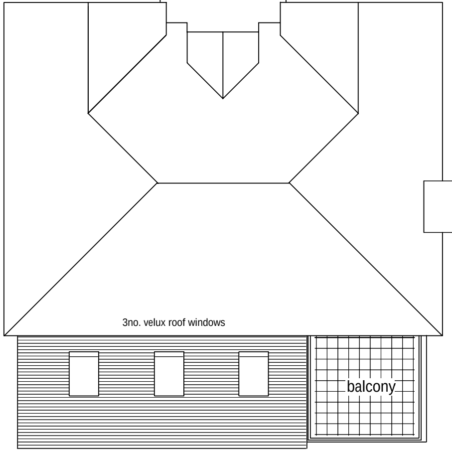
Prop. Roof Plan
