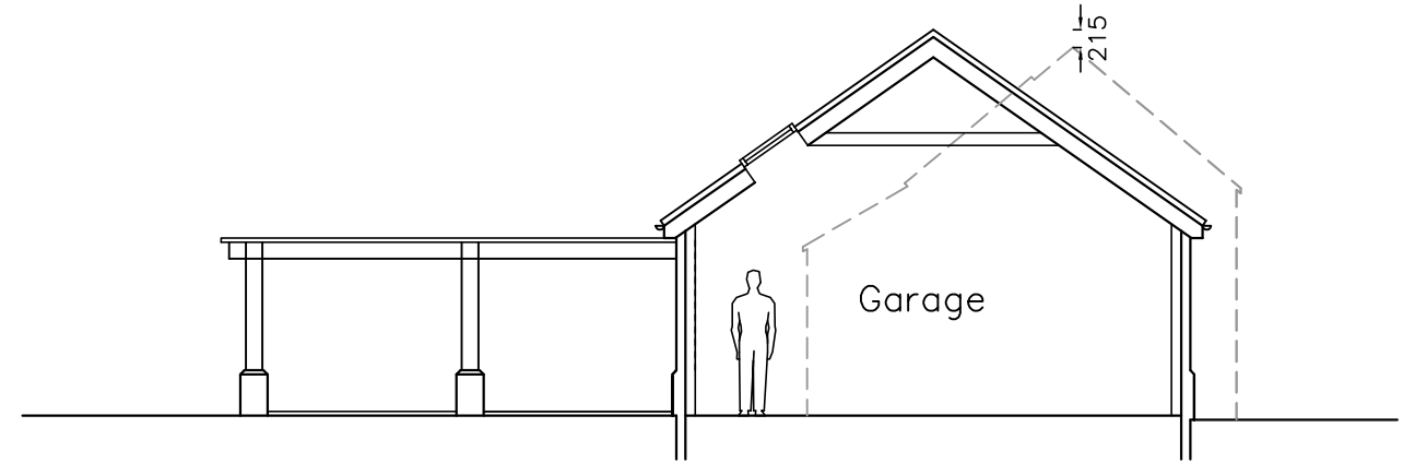
DRAFT SECTION
