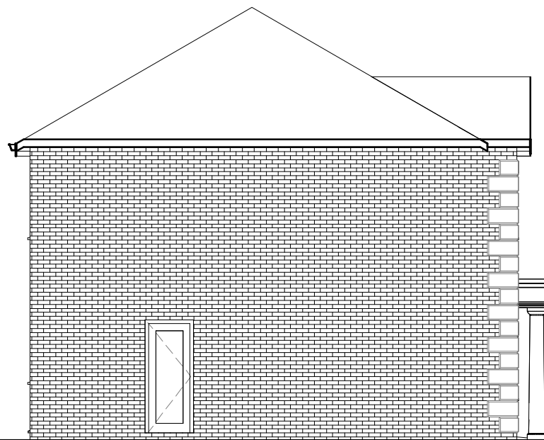
5 Elevation North HT D 1 : 100
