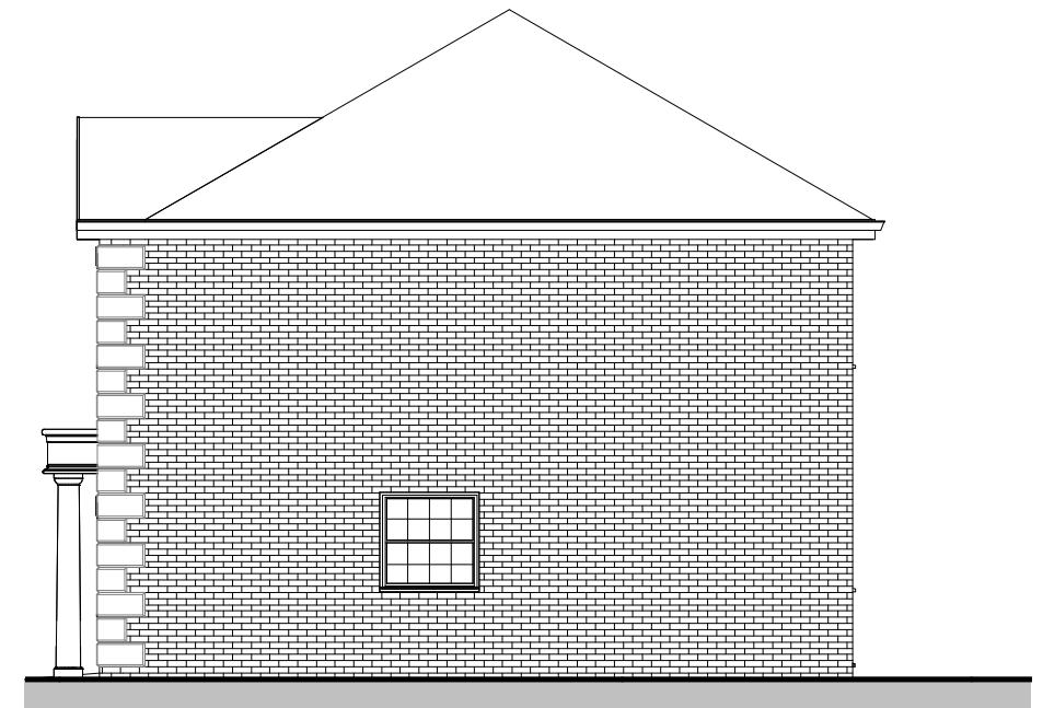
3 Elevation South HT D 1 : 100
