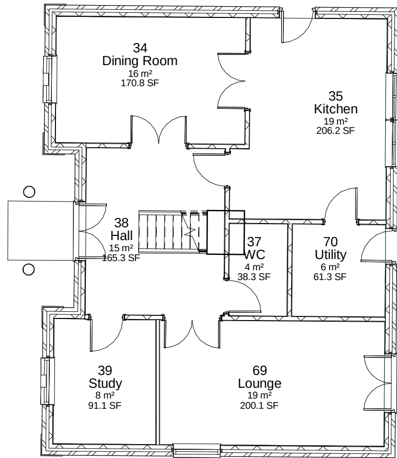
1 Ground Floor House Type D 1 : 100
