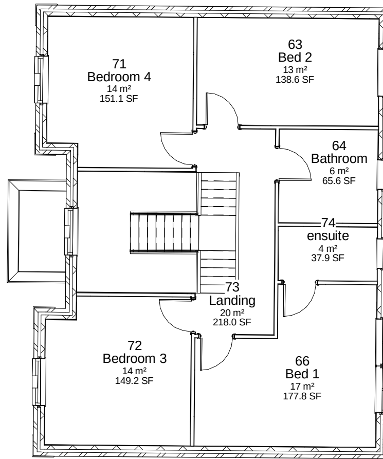
2 First Floor House Type D 1 : 100
