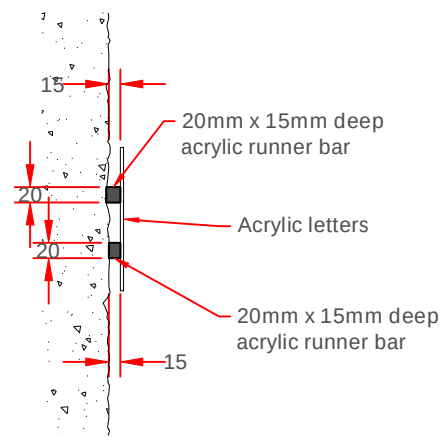
Letters Cross Section Scale 1:10 @A3
