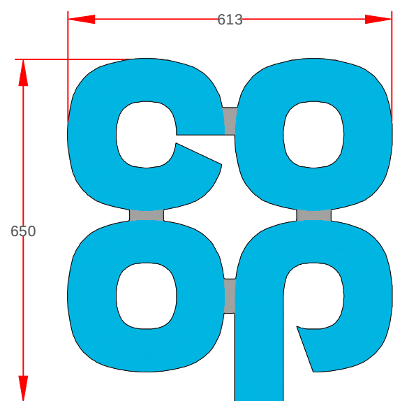
650mm Scale 1:10 @A3
