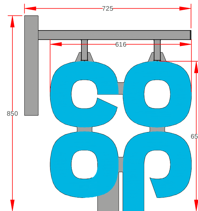
650mm Scale 1:10 @A3
