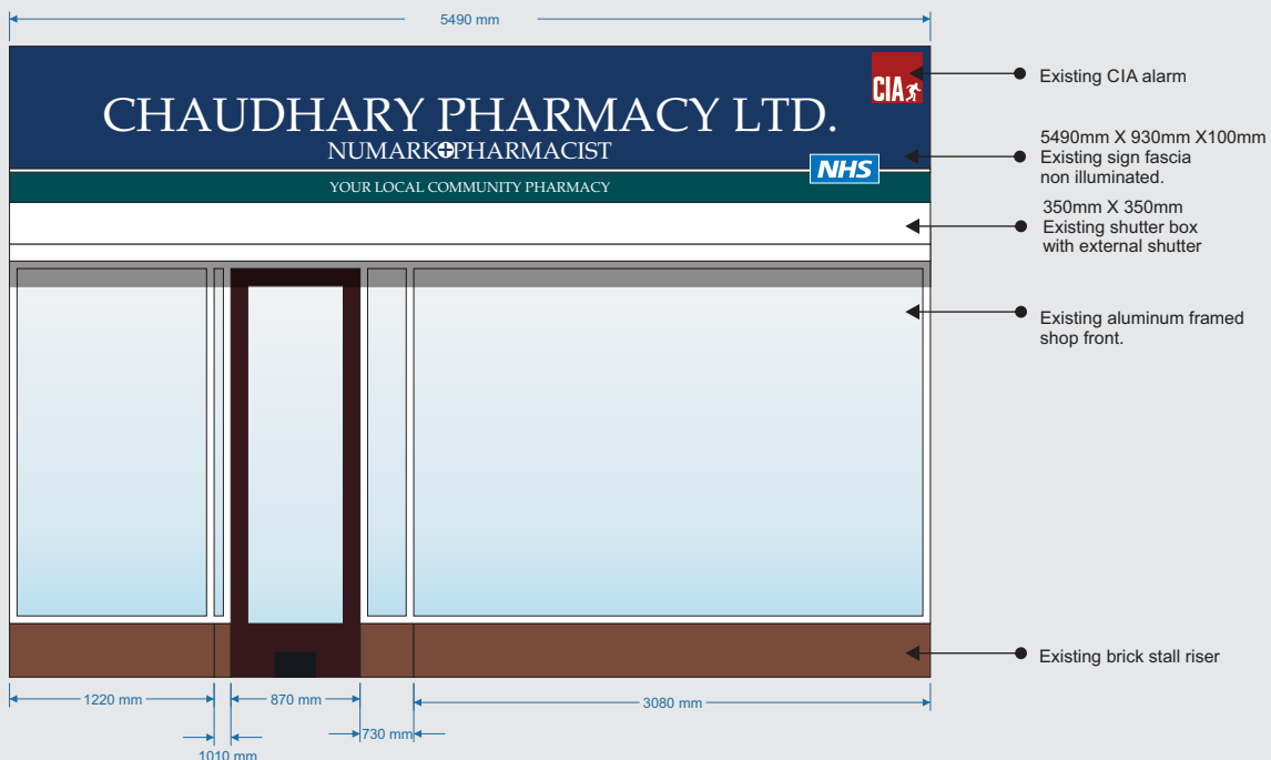
Existing Shopfront Elevation View
