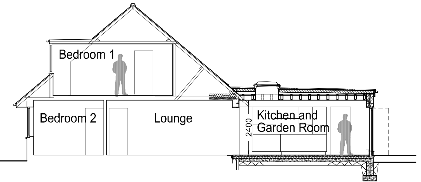
Section A - A as Existing 1:100
