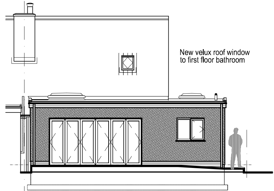
Rear (South) Elevation as Existing 1:100
