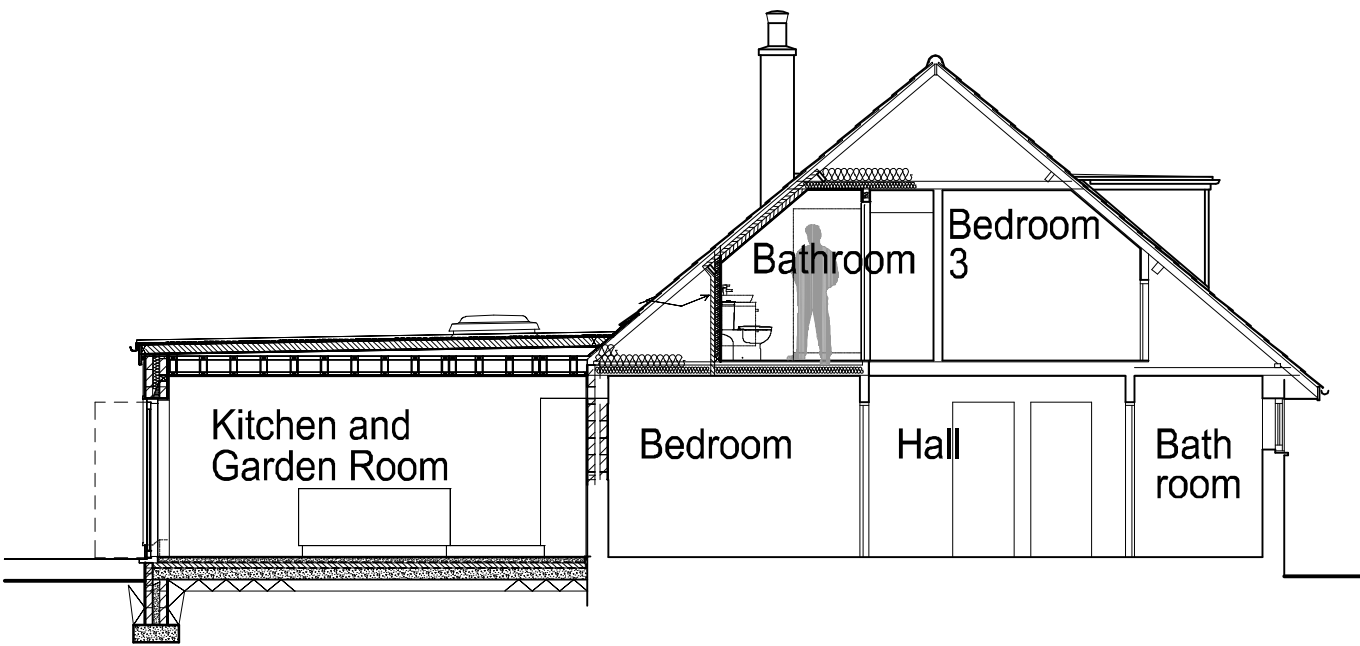
Section B - B as Existing 1:100
