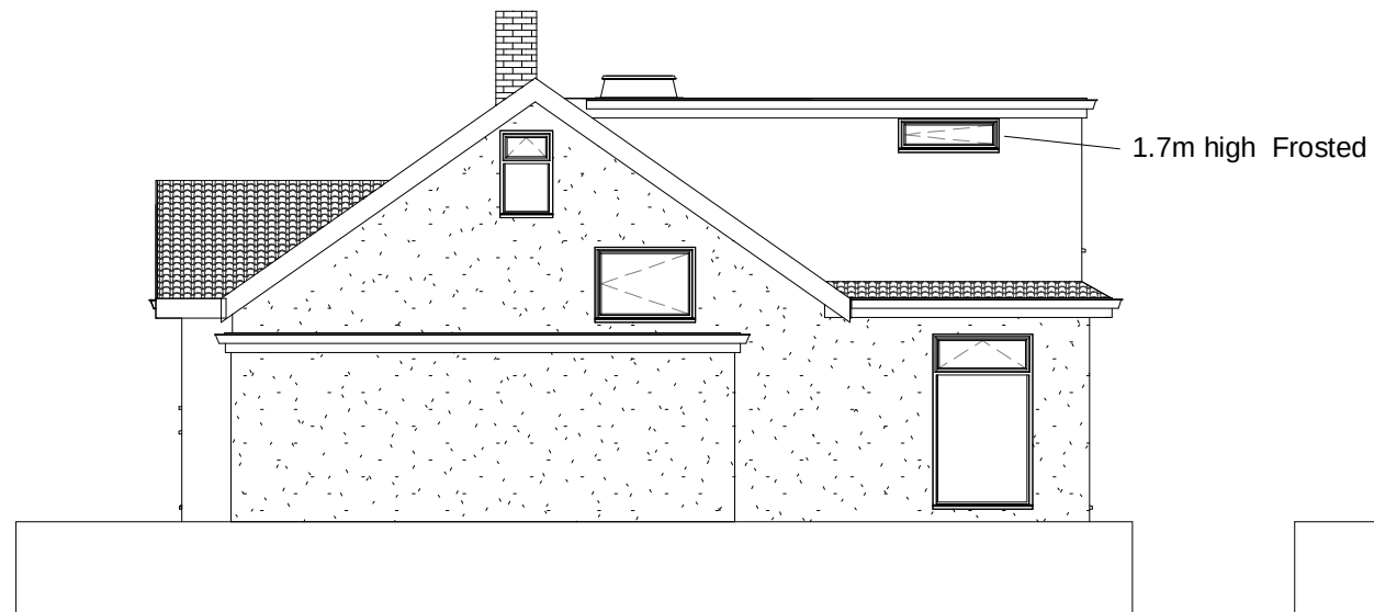
1 East Elevation 1 : 100
