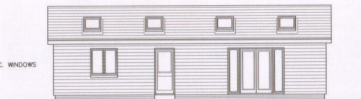
SIDE ELEVATION
