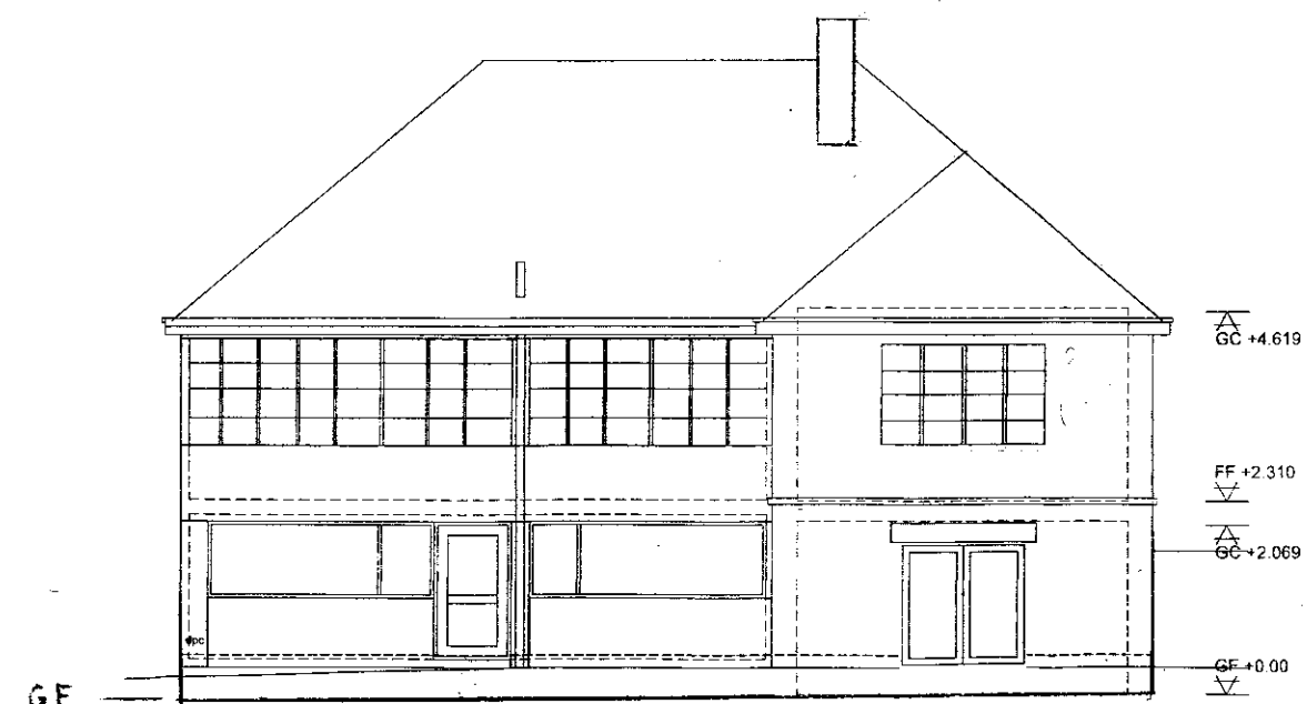
NORTH ELEVATION
