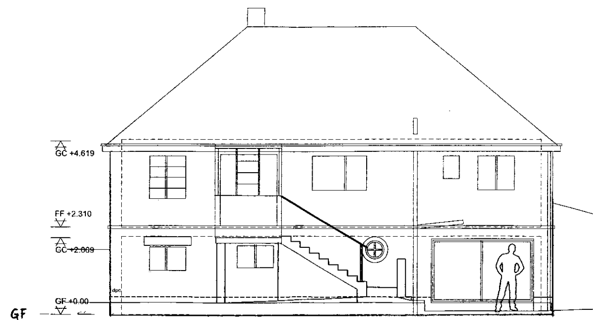
SOUTH ELEVATION
