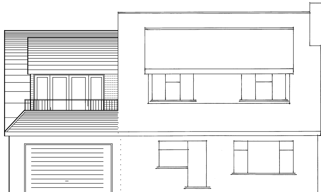
Proposed West/Front Elevation
