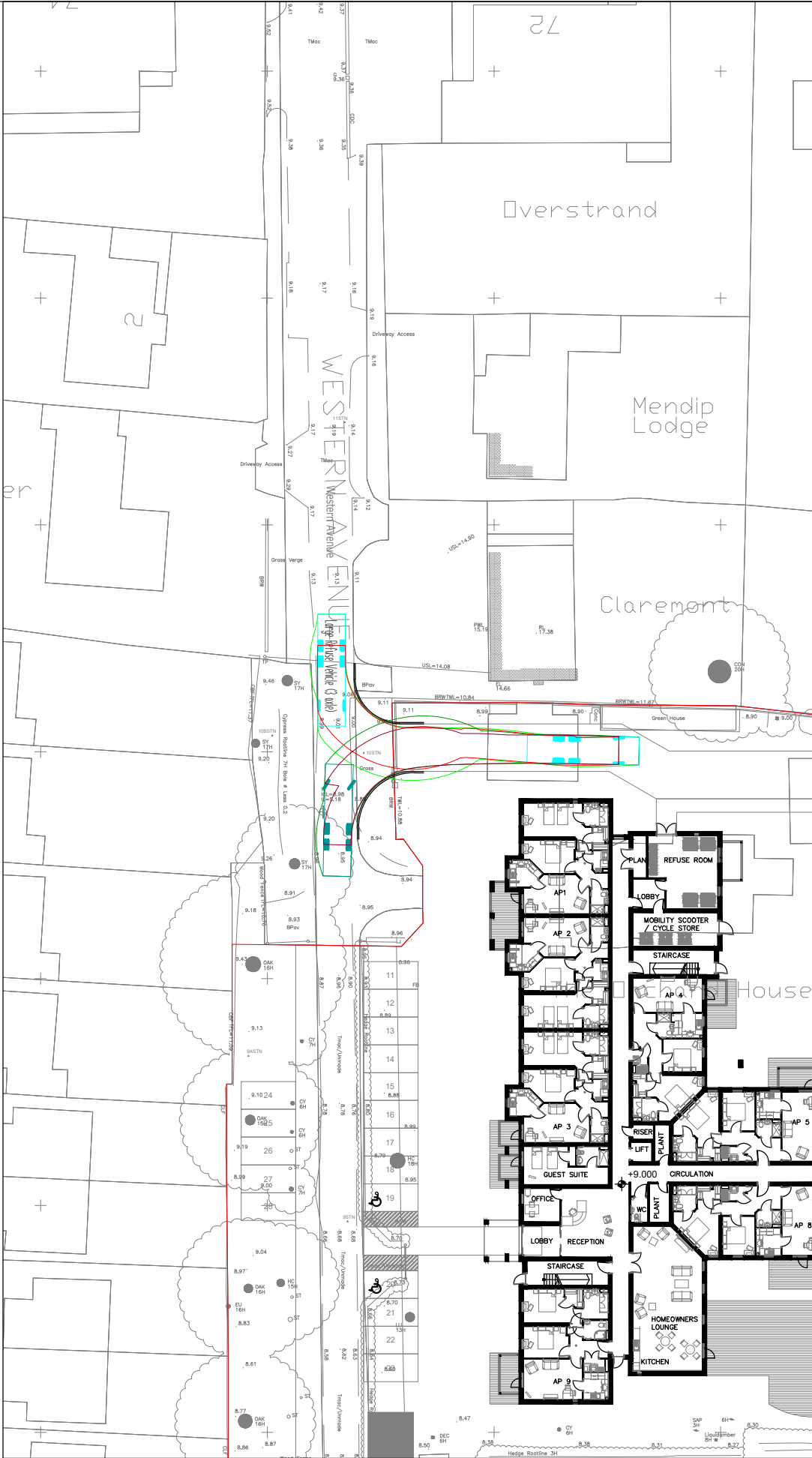
VEHICLE TRACKING
