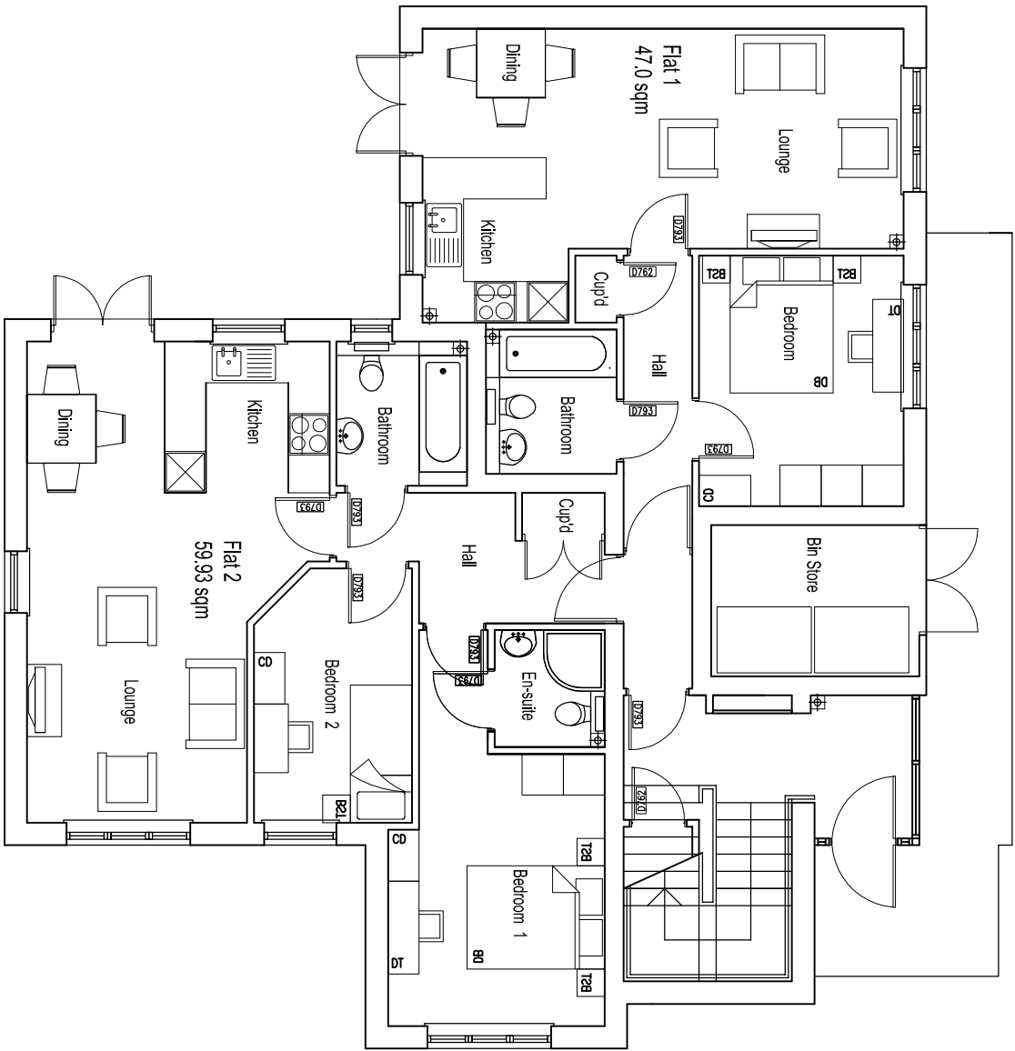
GROUND FLOOR
