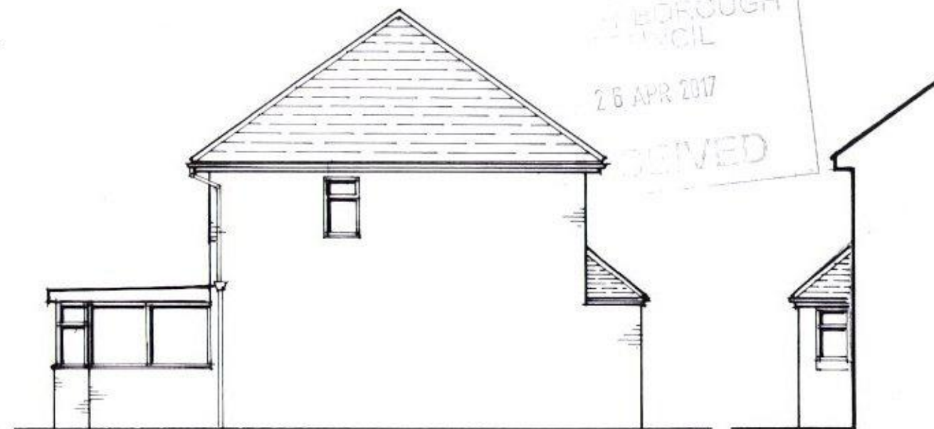
North Elevation
