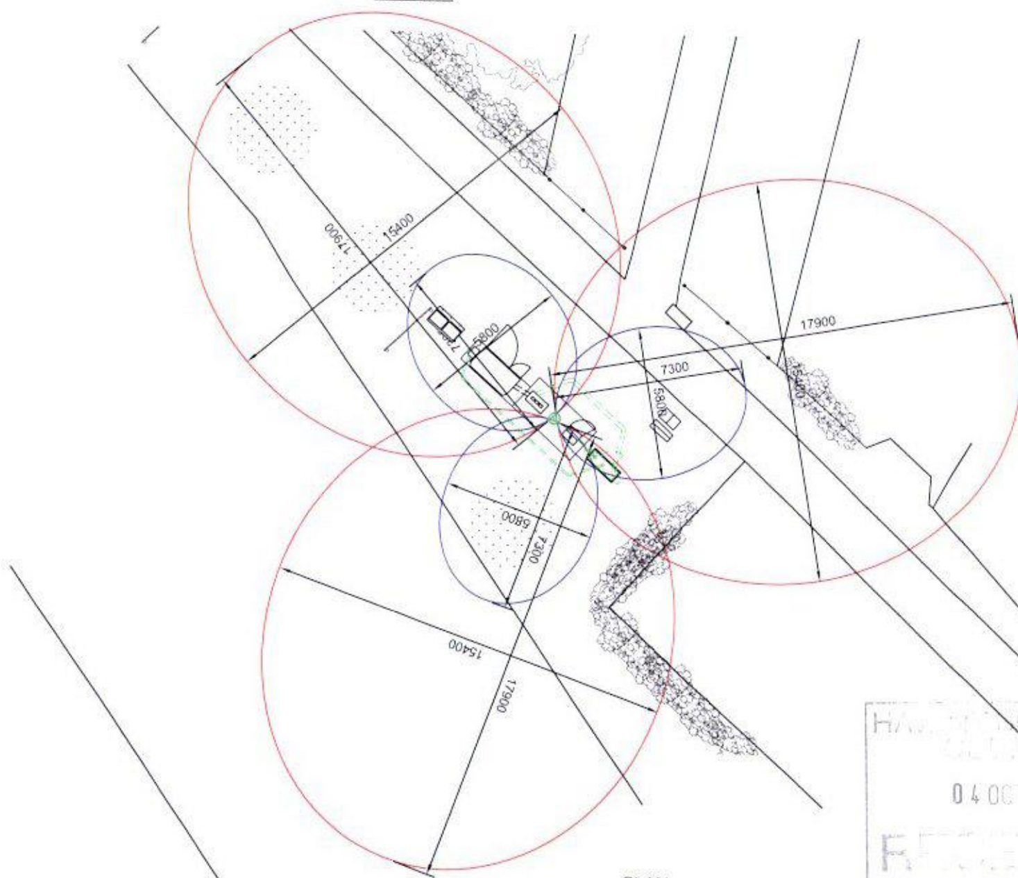
PLAN SCALE 1:200
