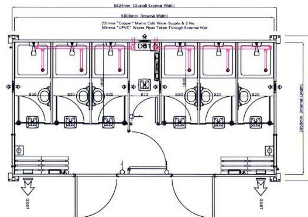
Floor Plan [Standard]
