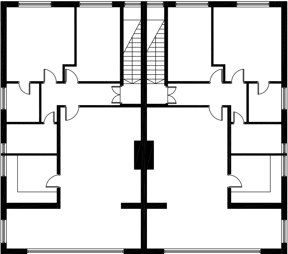
Existing First Floor Plan @ 1:100 Scale
