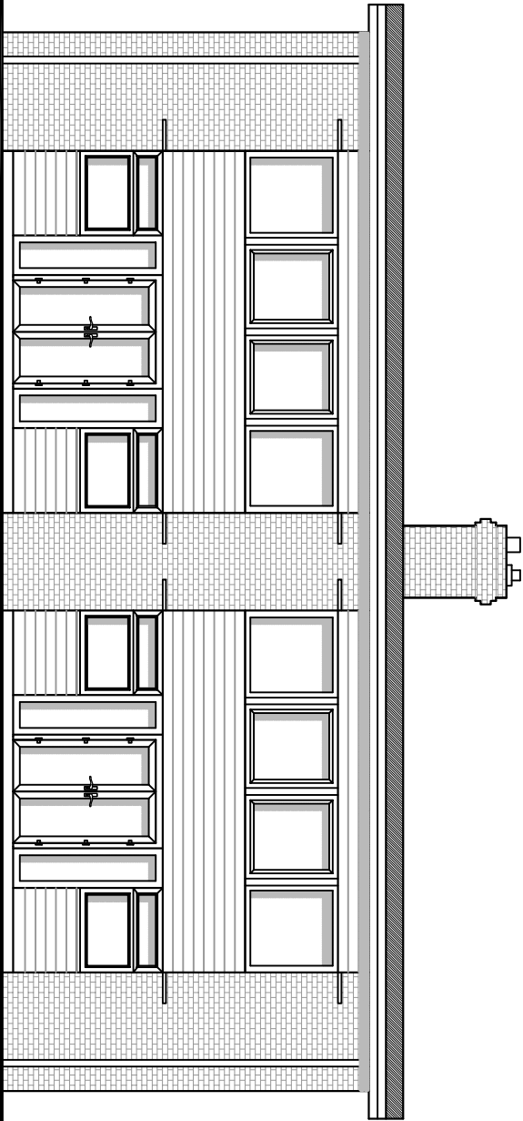
Existing South Elevation @ 1:100 Scale
