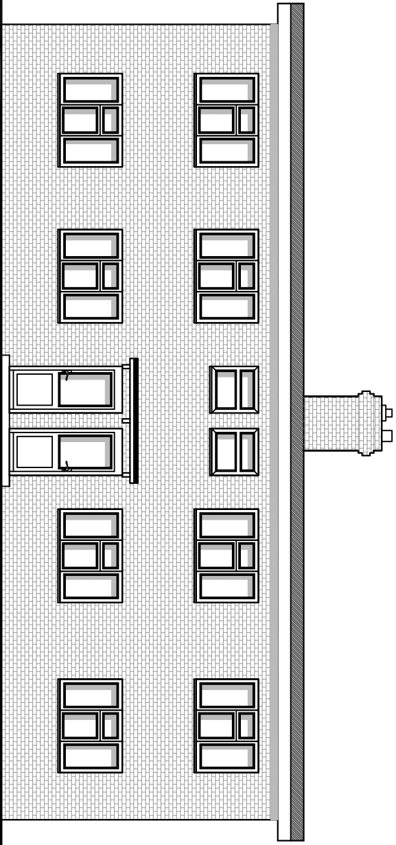
Existing North Elevation @ 1:100 Scale
