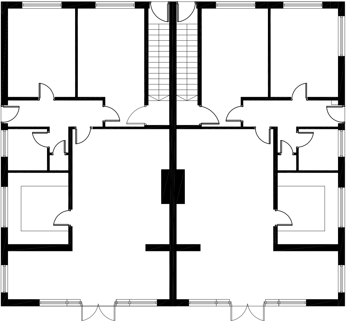
Existing Ground Floor Plan @ 1:100 Scale
