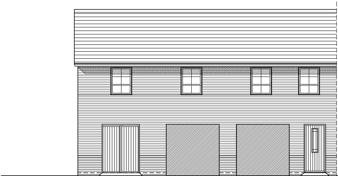
Front Elevation
