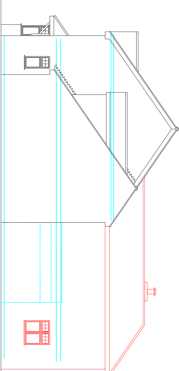
Proposed Side Elevation (north)
