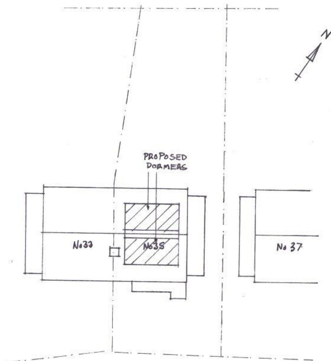
BLOCK PLAN
