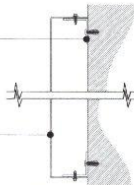
SECTION THRO' SIGNS 1:5 SCALE @ A4
