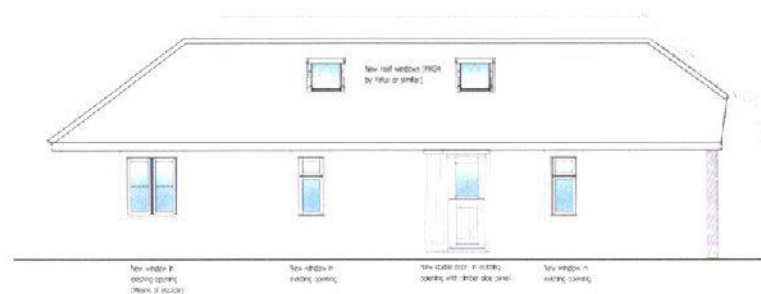
Proposed South (Front) Elevation
