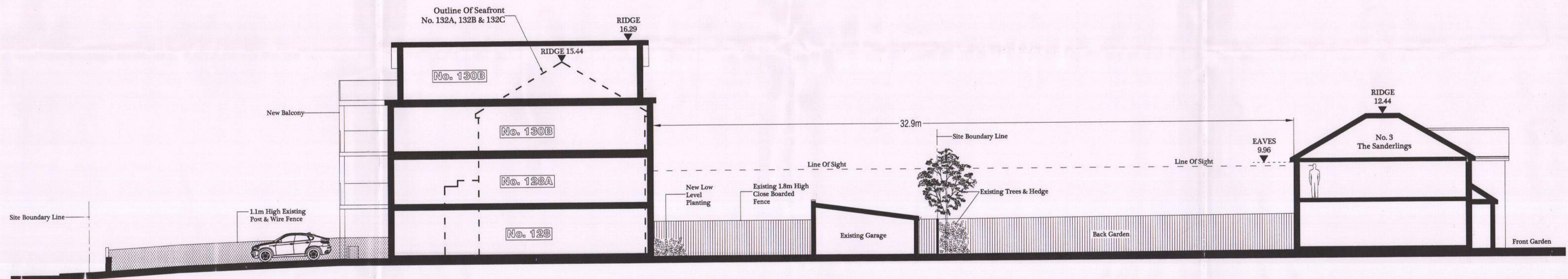
Proposed Site Section D-D @ 1:100
