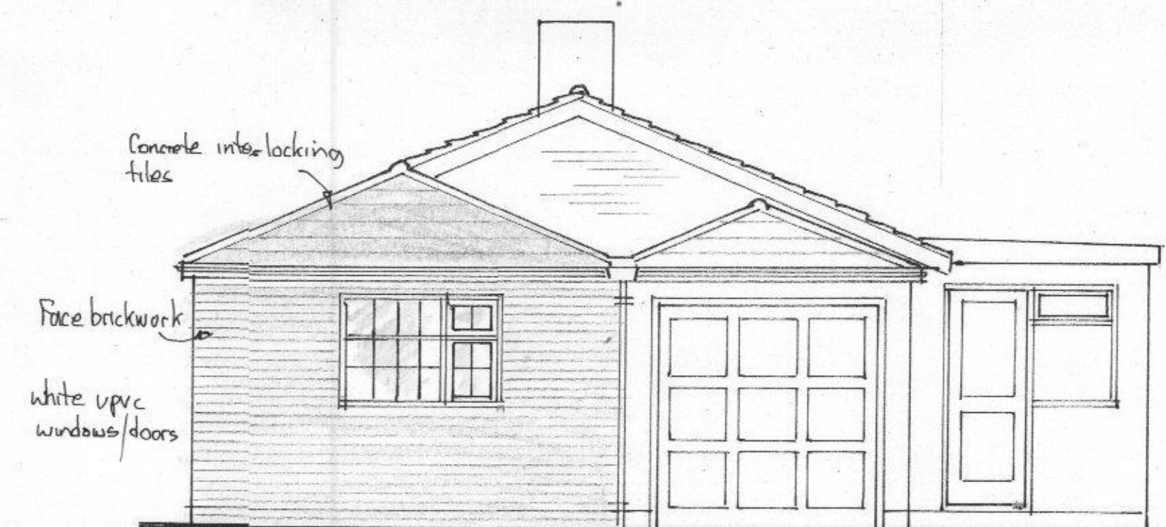
SIDE ELEVATION
